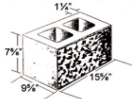
10x8x16 STANDARD*
