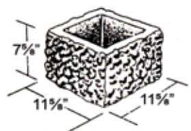
12x8x12 COLUMN
