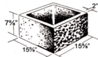
16x8x16 DOUBLE "C" PILASTER*
