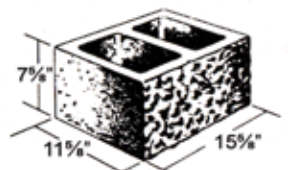
12x8x16 STANDARD*
